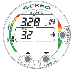
Fig. 4.17. Setting Nitrox parameters. Oxygen percentage is 32%, oxygen partial pressure limit is 1.4 bar. The equivalent maximum depth is displayed as 32.8 m [107 ft]. Press scroll buttons to change oxygen percentage and to set oxygen partial setting value. Accept settings by pressing MODE (OK).
