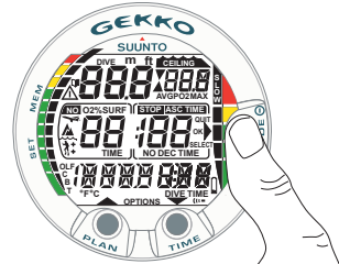
Fig. 3.1. Startup I. All segments shown.
